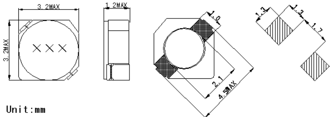
Land Pattern
