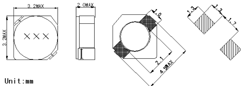
Land Pattern
