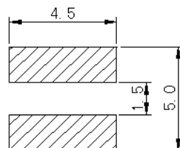
Land Pattern
