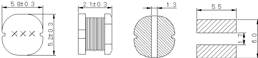
Land Pattern
